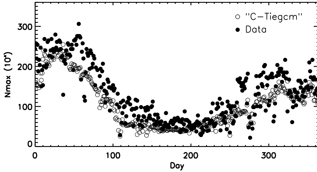
CHILTON Noon NmF2 C.DEVP7
