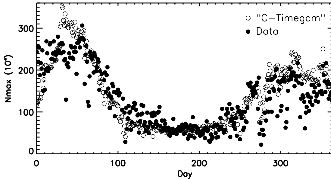
CHILTON Noon NmF2 C-TIEGCM
